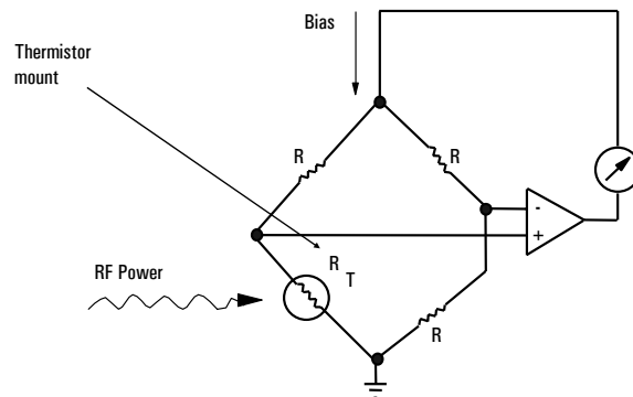
A self-balancing bridge containing a thermistor
