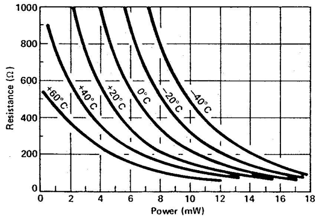
Characteristic curves of a typical thermistor element
